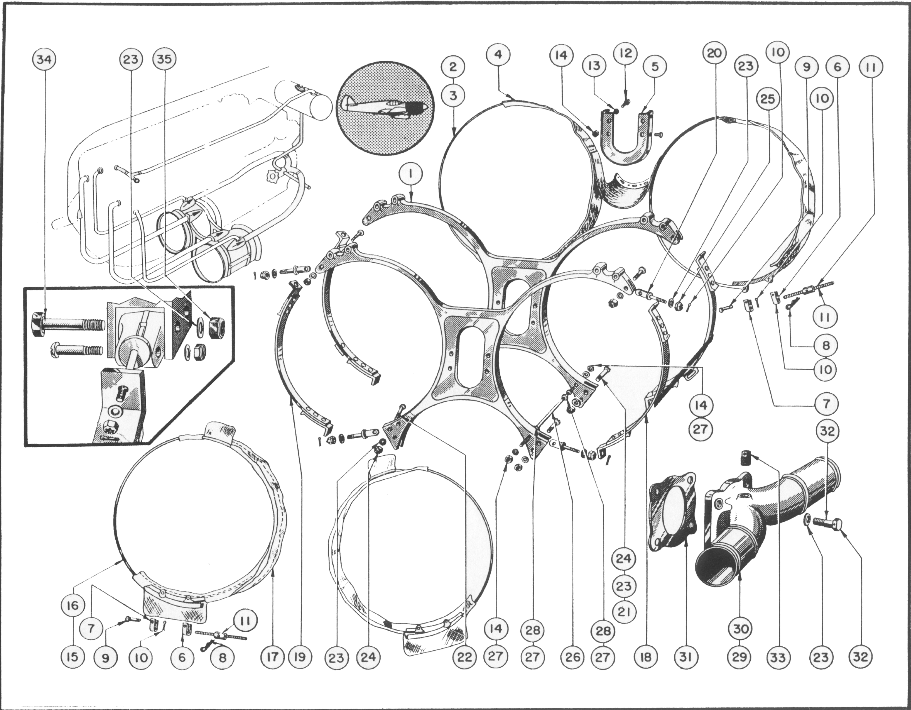
Figure 84—Coolant System
