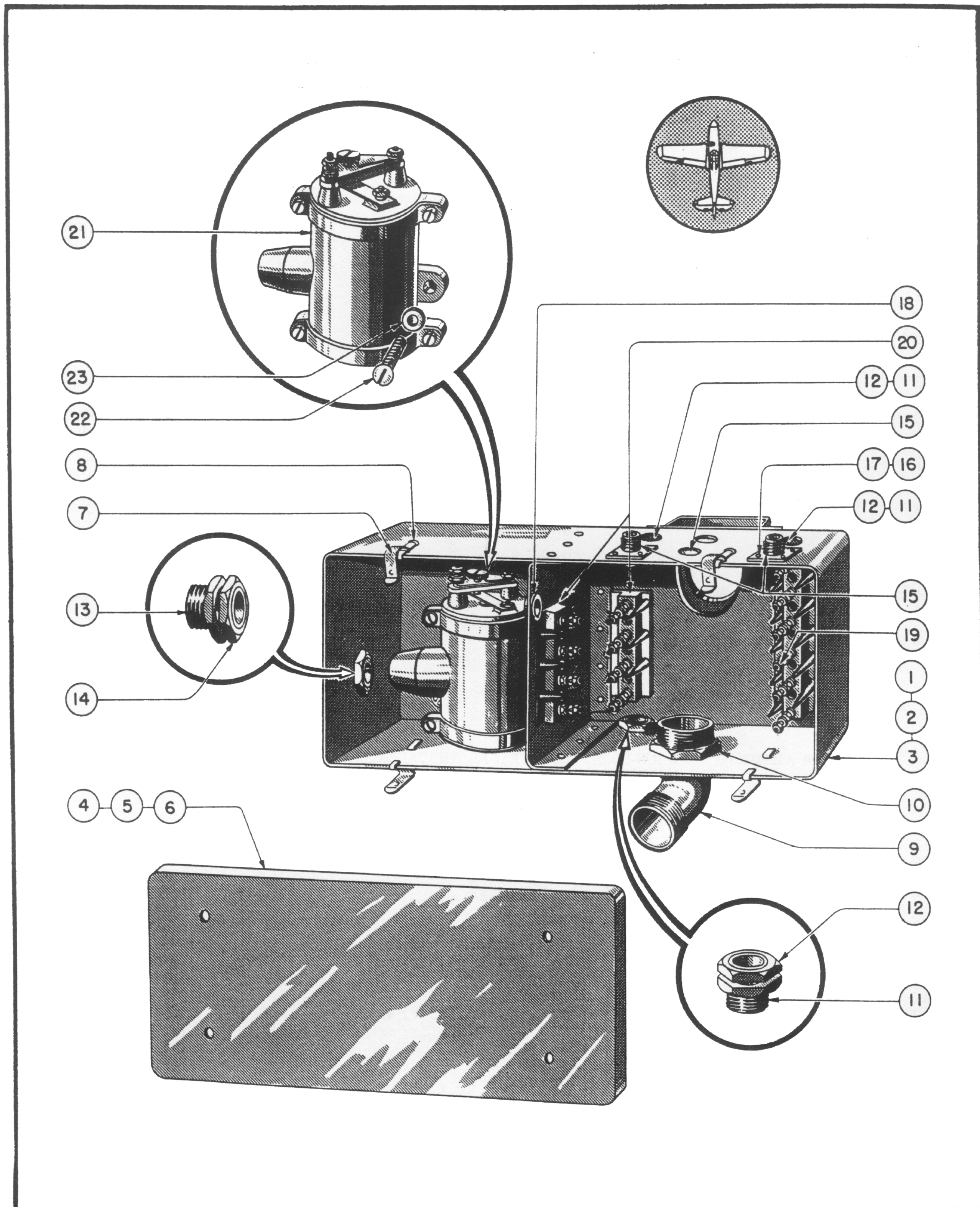
Figure 87—Firewall Terminal Box
