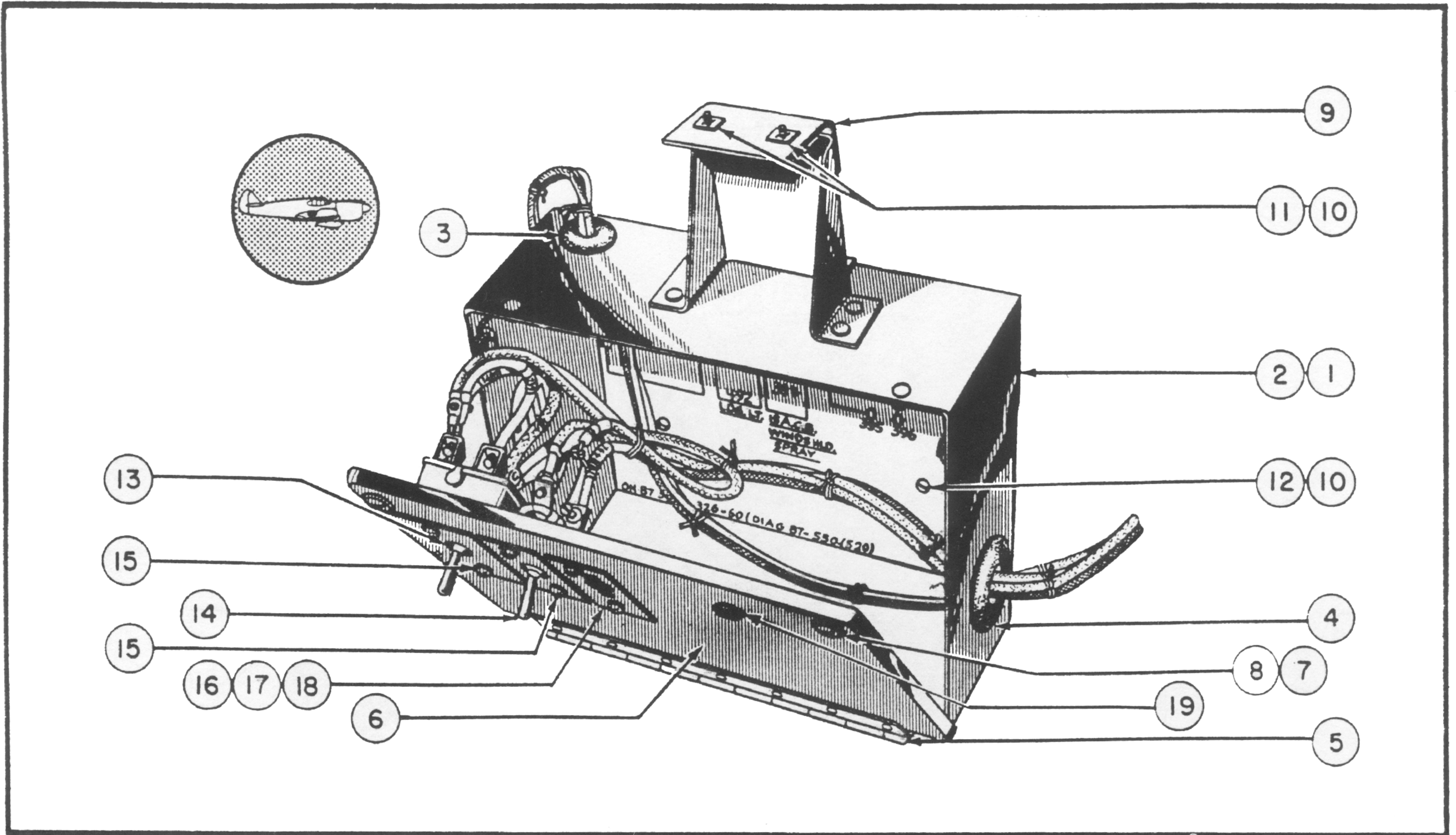
Figure 88—Winterization Junction Box Installation
