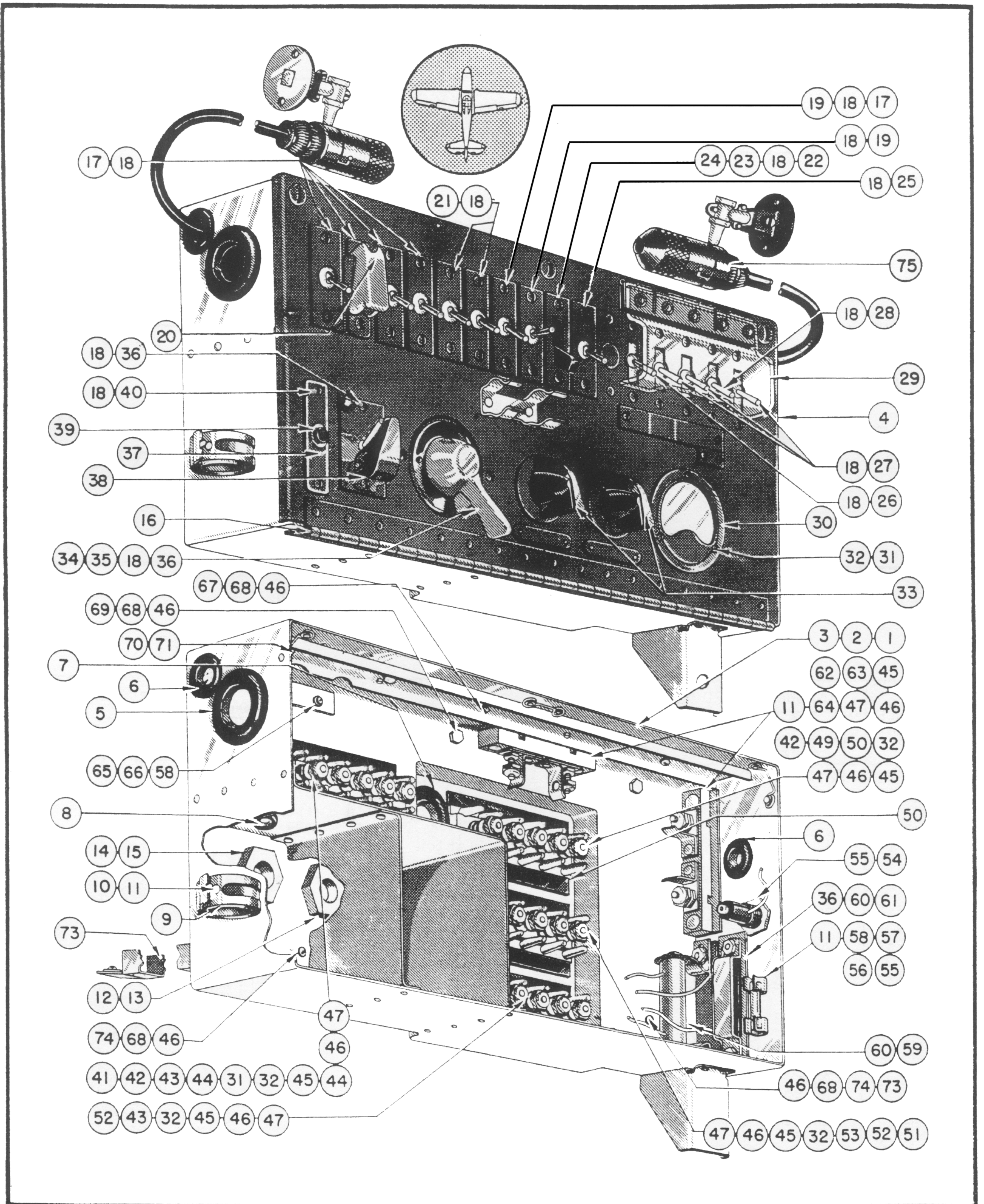
Figure 89—Main Switch Box Installation
