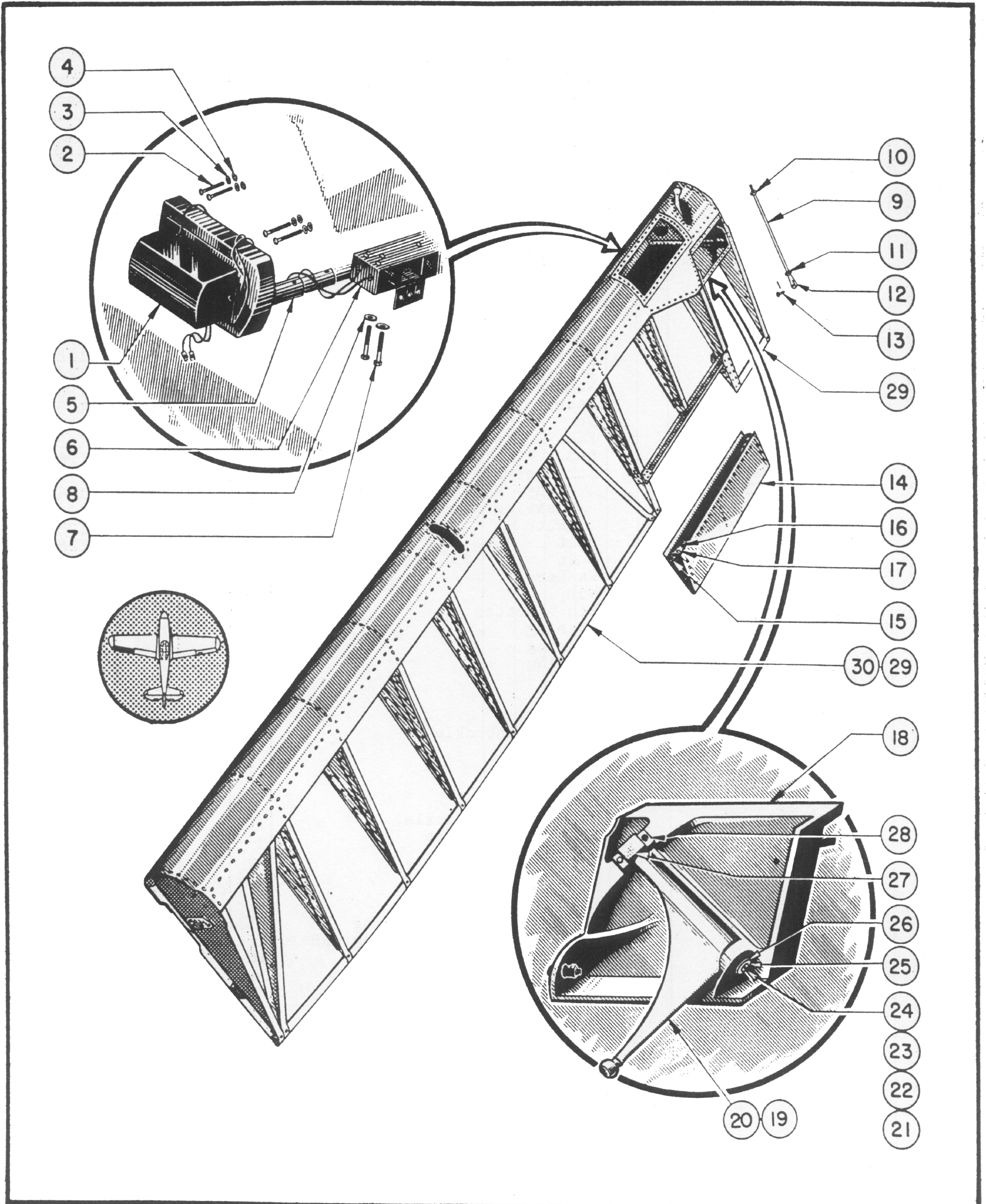
Figure 9—Left Hand Aileron Assembly
