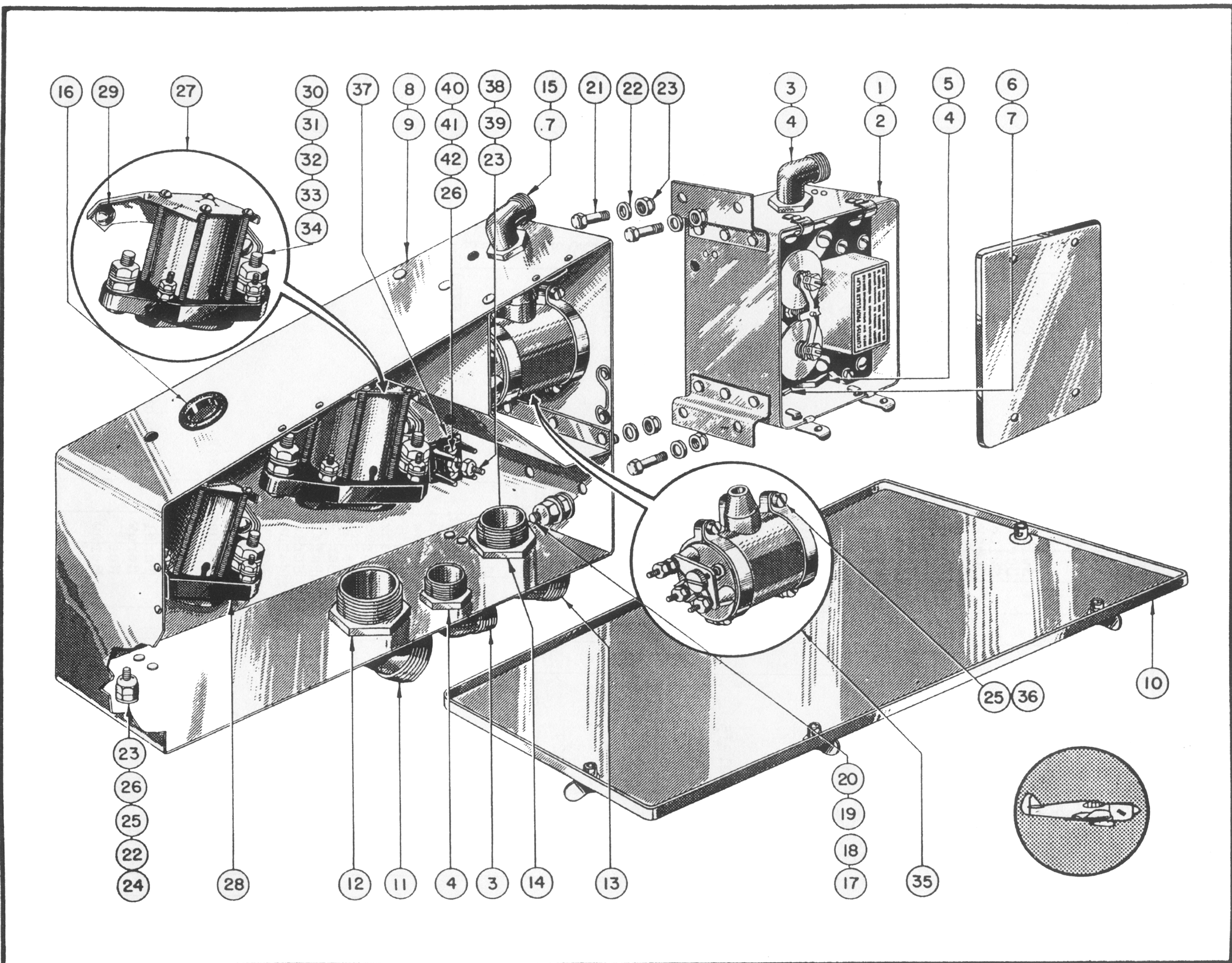
Figure 90—Battery Junction and Propeller Relay Boxes Installation
