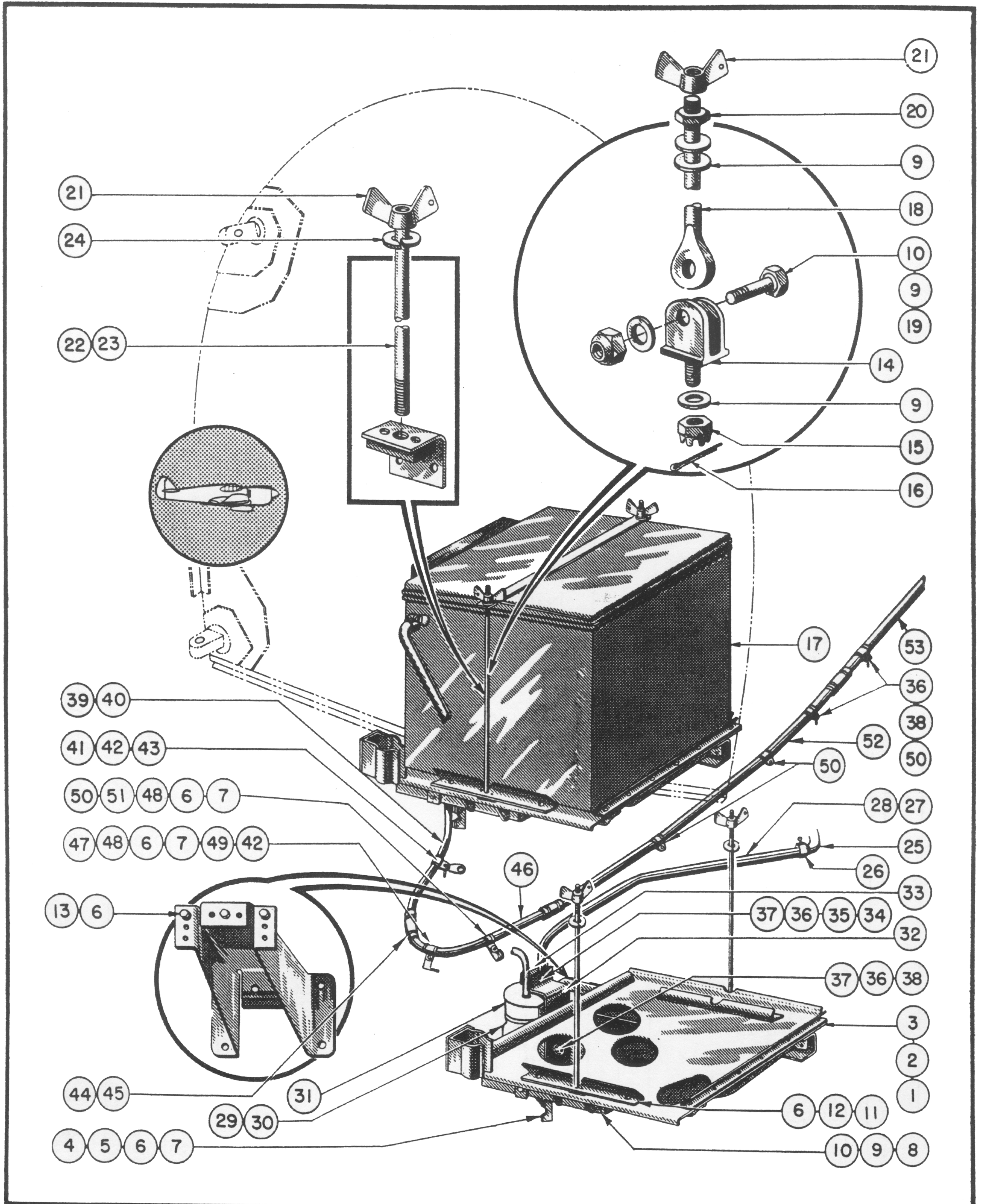
Figure 91—Forward Firewall Battery Installation
