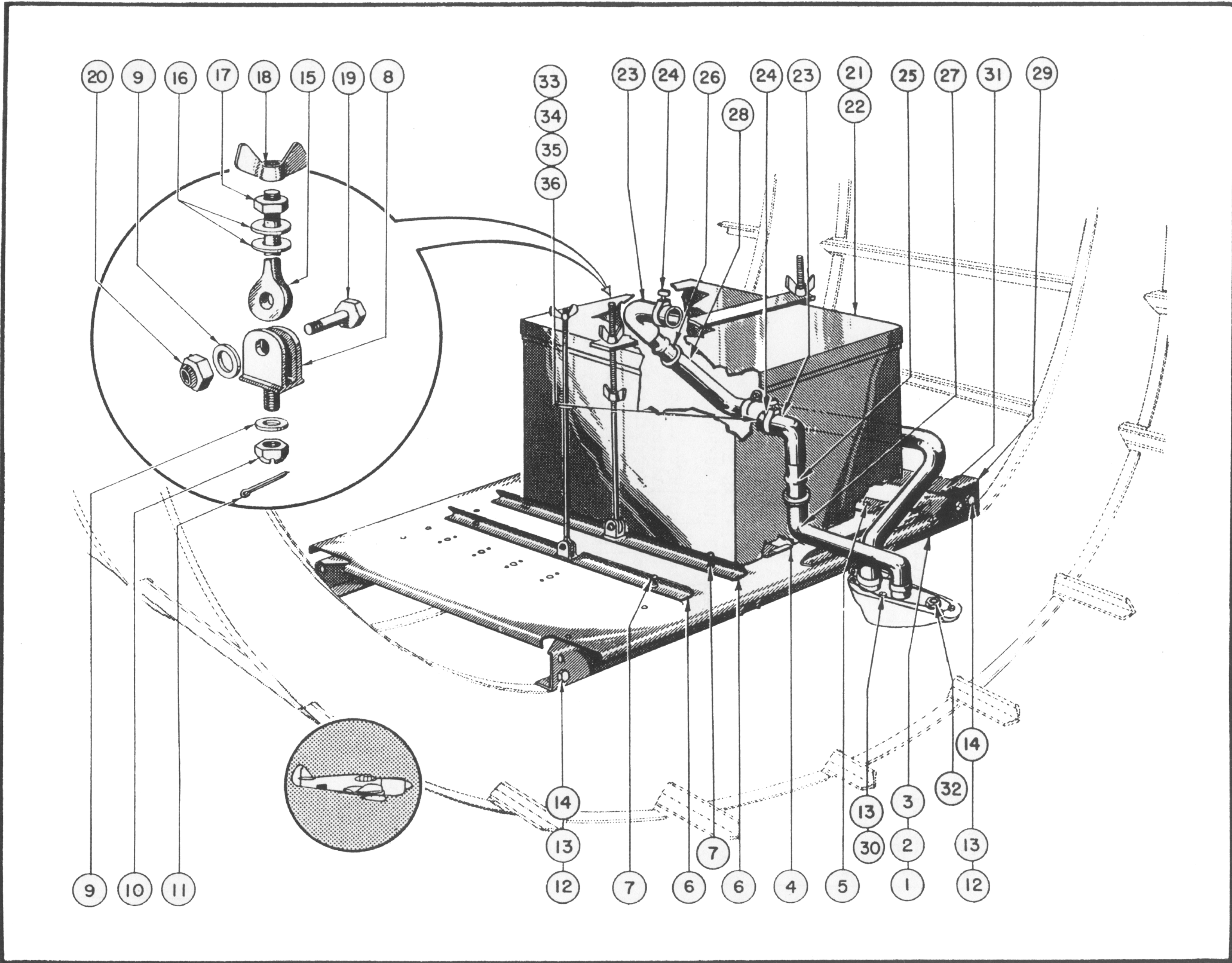
Figure 92—Battery & Hydraulic Pump Support Installation
