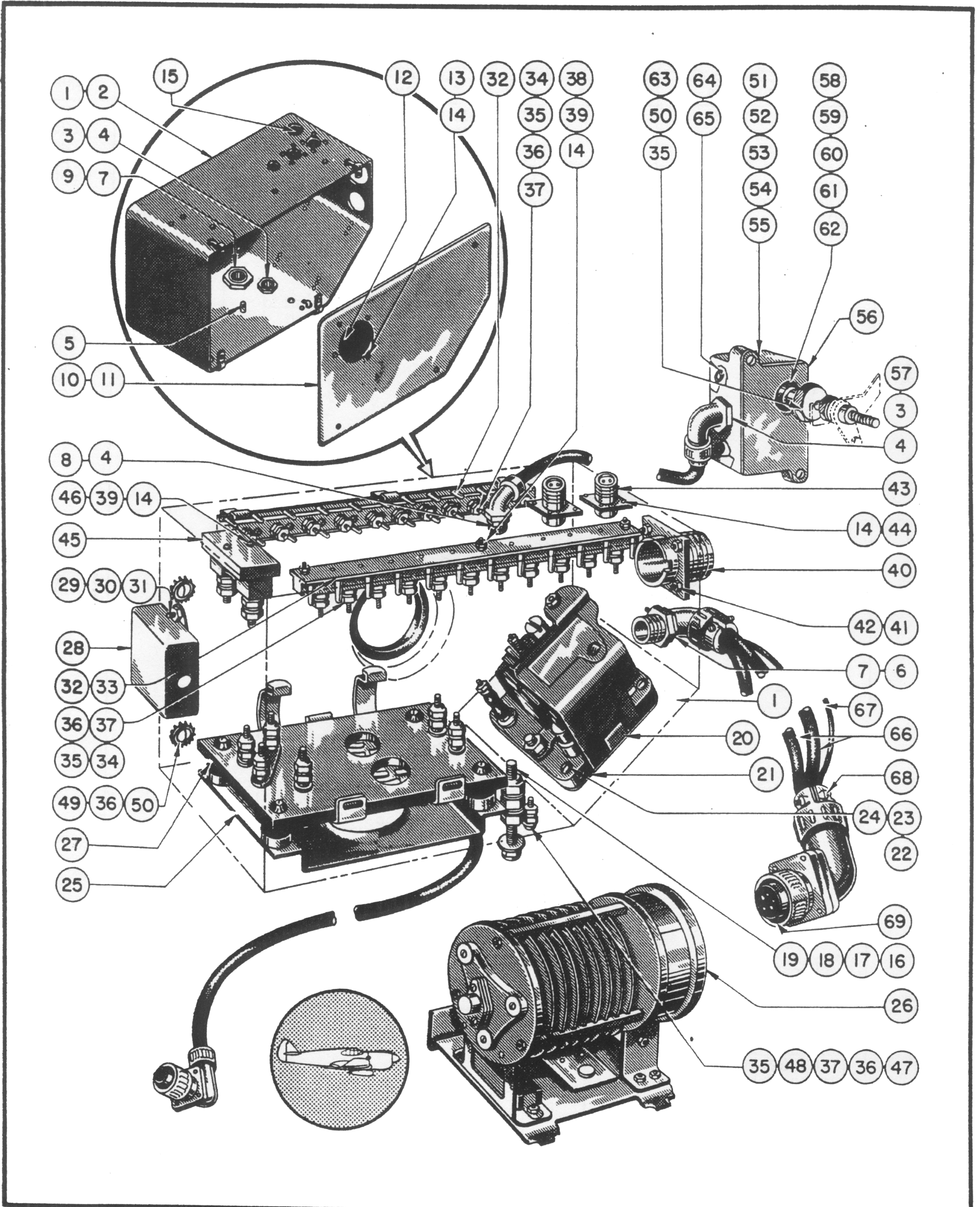
Figure 93—Firewall Junction Box & Landing Gear Warning Switch Installation
