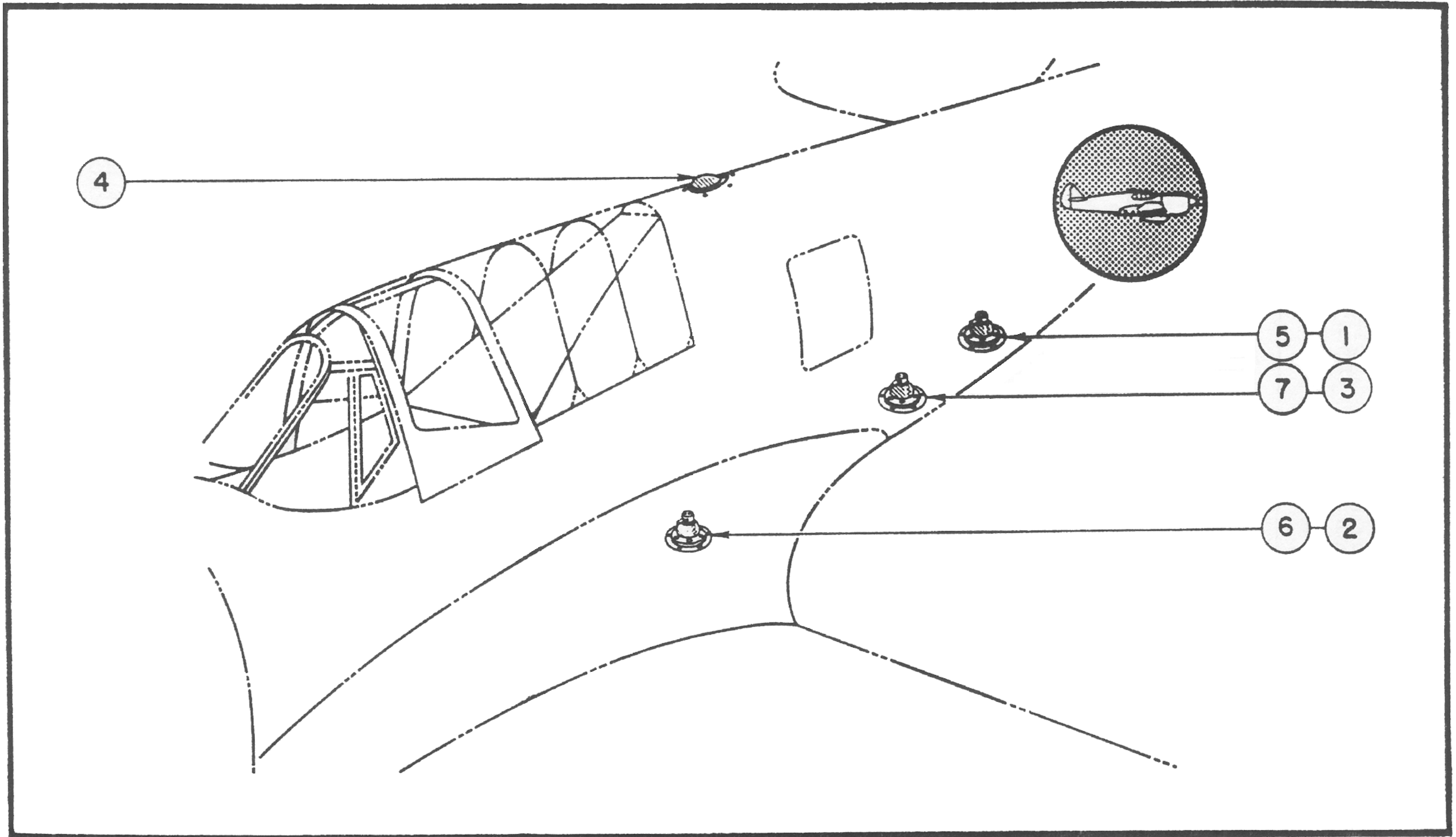
Figure 94—Fuselage Electrical Installation
