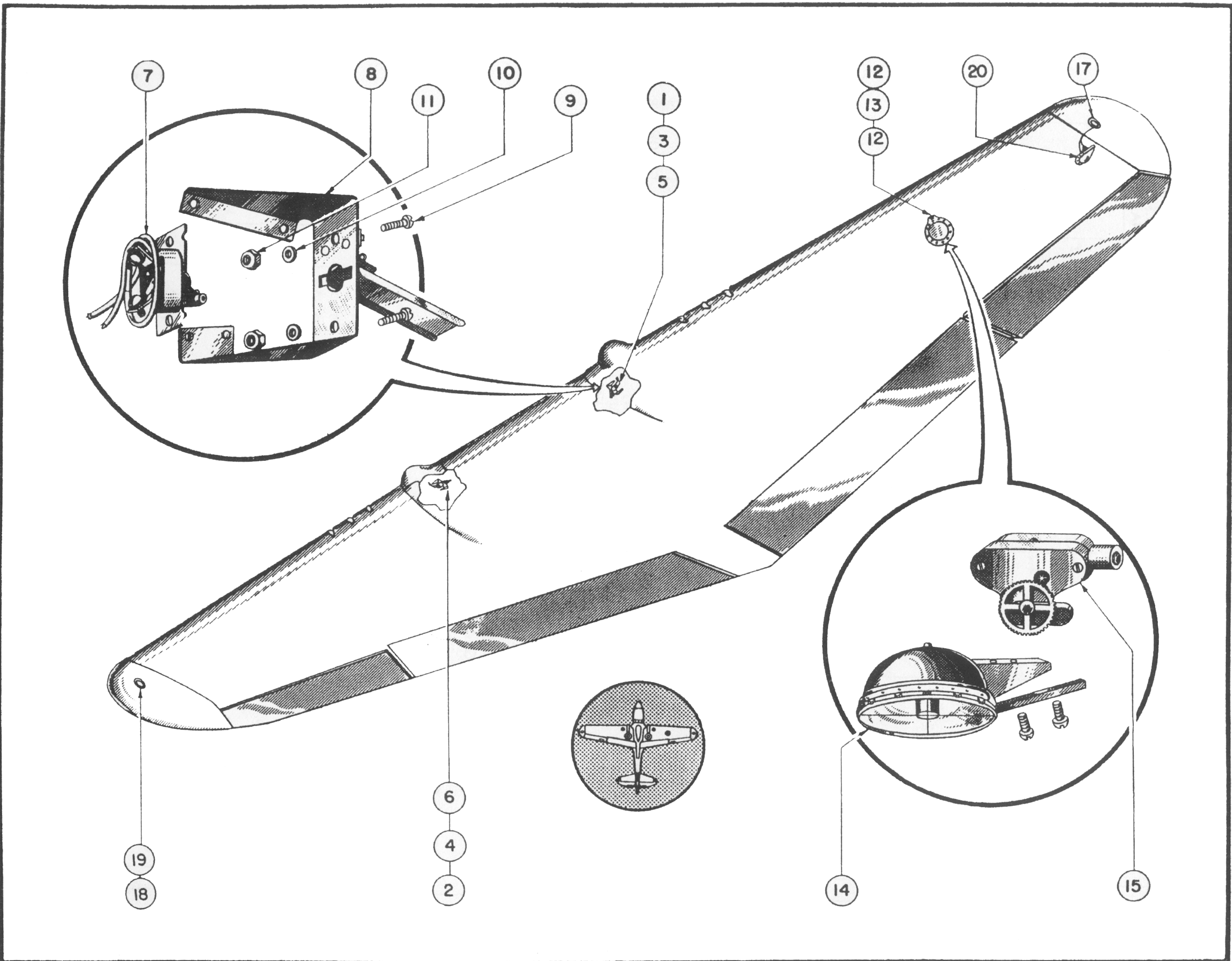
Figure 95—Wing Panel Electrical Installation
