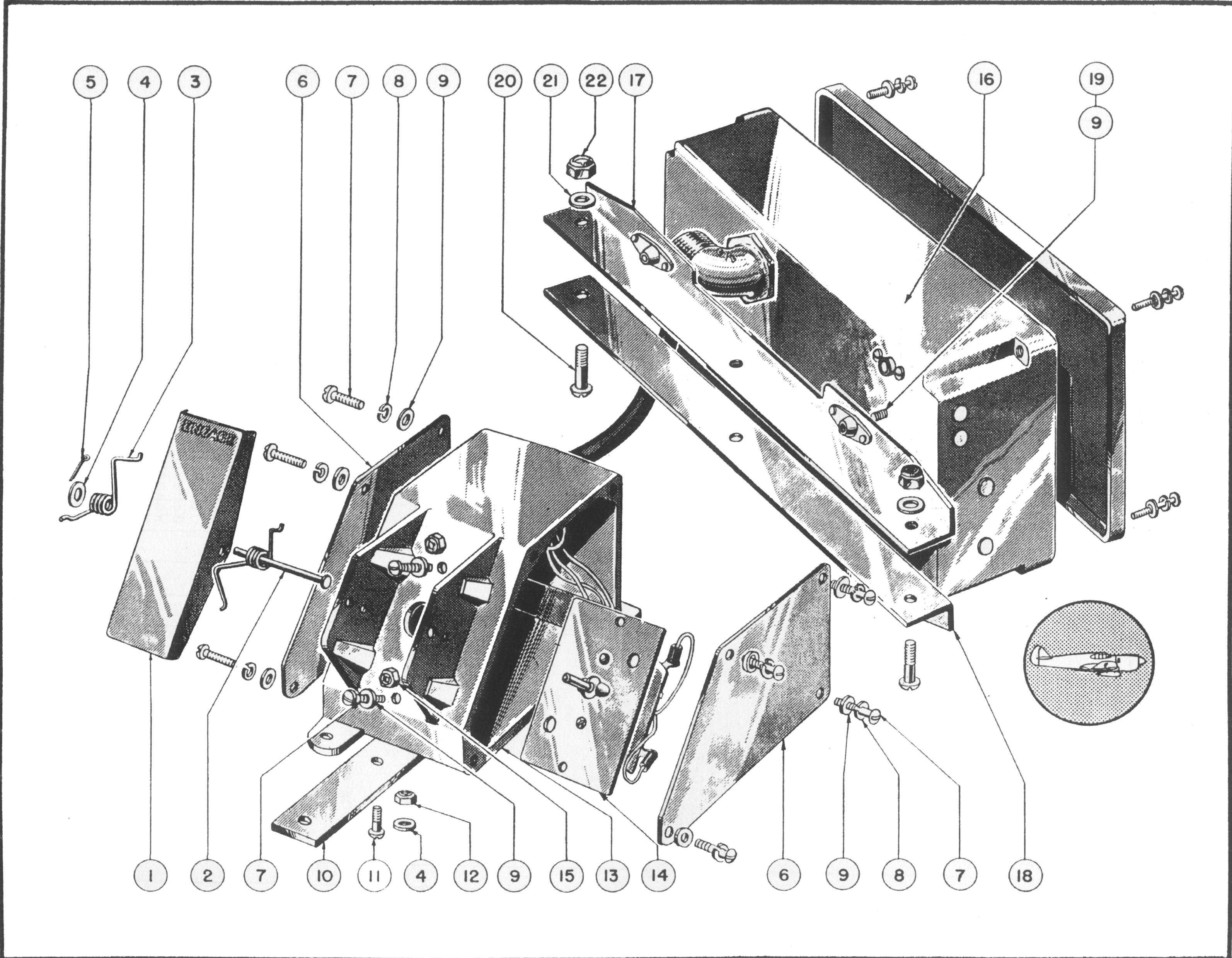
Figure 96—Starter Pedal and Stick Box Installation
