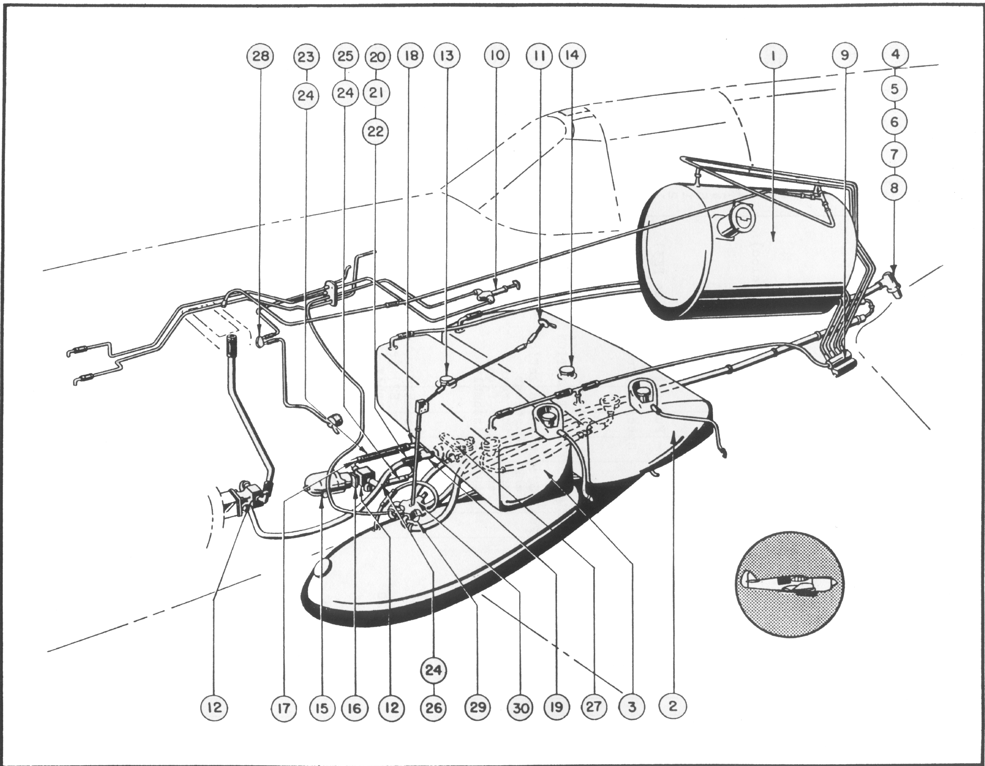
Figure 99—Fuel System Installation (F-W)
